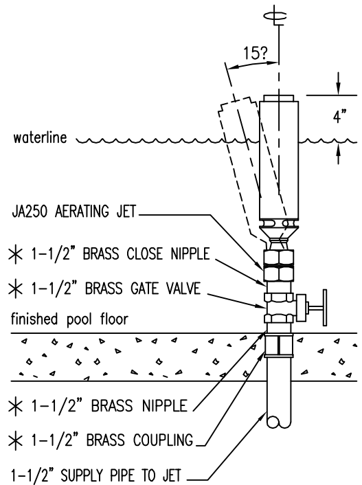
Typical Installation Detail
